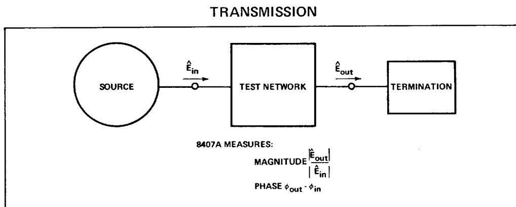
Figure 1-1. Transmission Diagram
