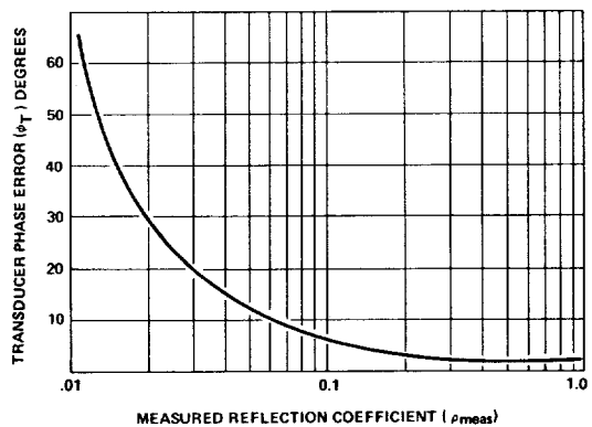
Figure 6-5. Plot of Transducer Phase Error ( \phi_T ) as a function of reflection coefficient.
