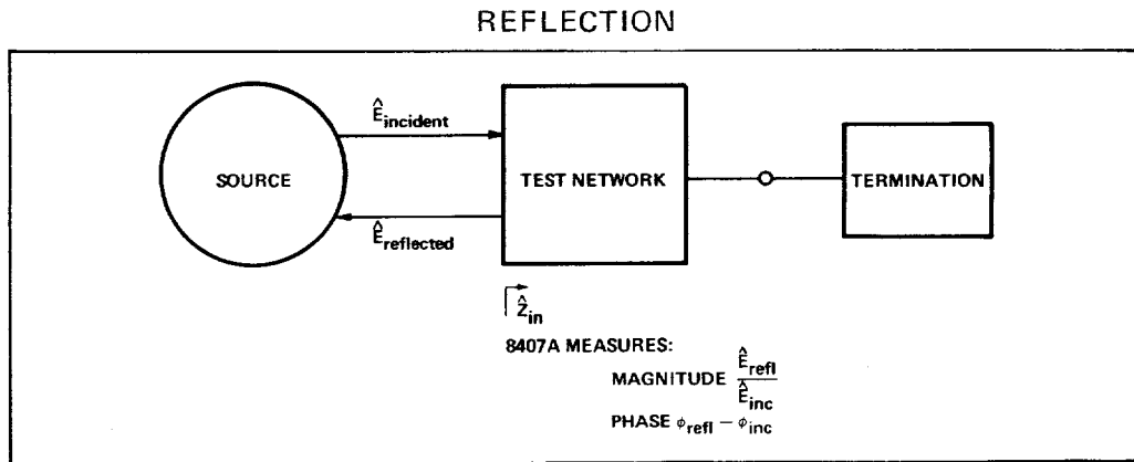
Figure 1-3. Reflection Diagram. The magnitude and phase of the reflected signal will depend upon the impedance looking into the input of the two-port network. For a more detailed treatment of signal flow graph analysis, ask your nearest HP sales office for AN 95.
